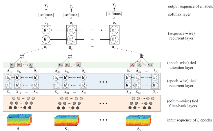
Illustration of SeqSleepNet, as described in the paper “SeqSleepNet: End-to-End Hierarchical Recurrent Neural Network for Sequence-to-Sequence Automatic Sleep Staging” by H. Phan, F. Andreotti, N. Cooray, O. Y. Chén, and M. De Vos on p. 400.
